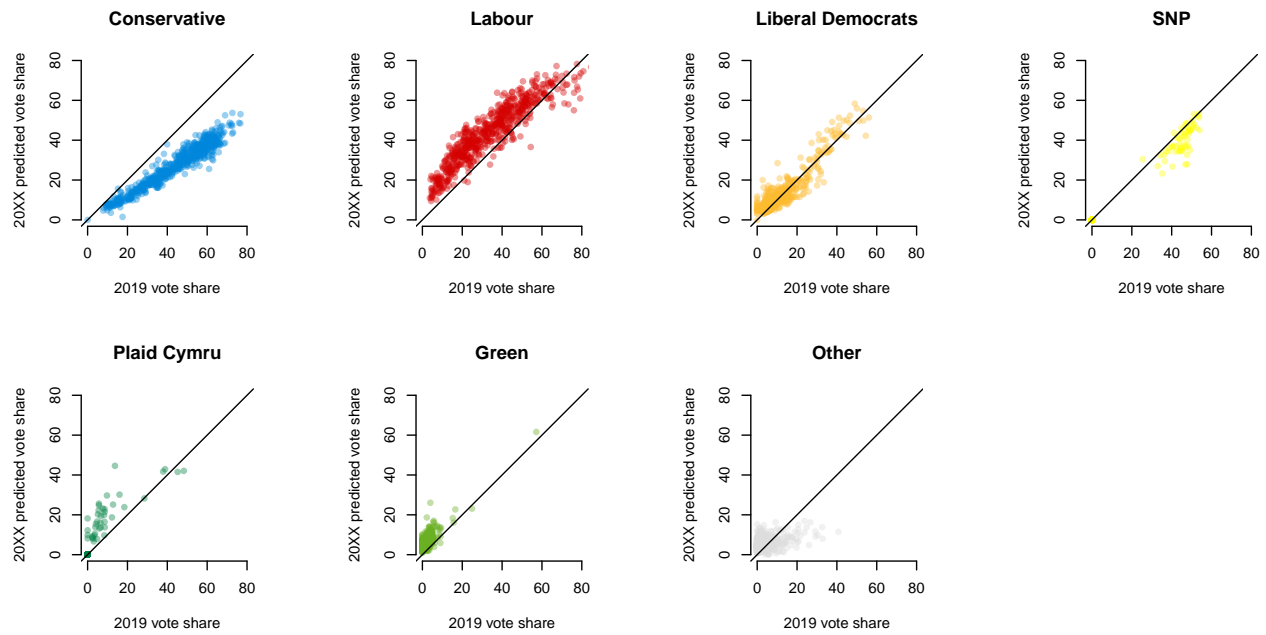
Figure 1: Predicted Constituency Vote Share by 2019 Constituency Vote Share
